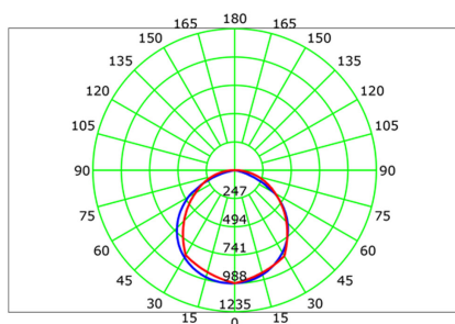
Luminous Intensity Distribution Curve
