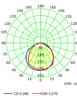
Luminous Intensity Distribution Curve
