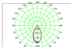
Luminous Intensity Distribution Curve
